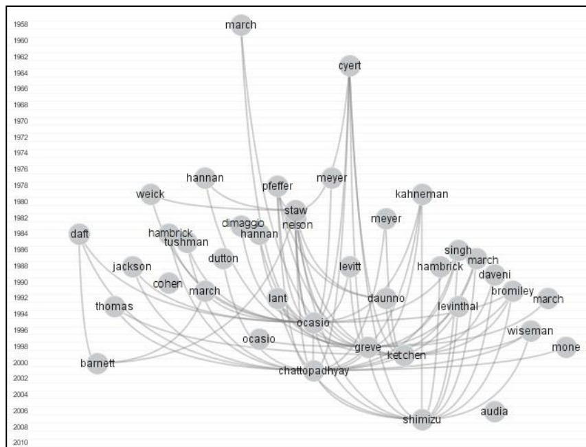
Figure 32 – Main co-citations.
